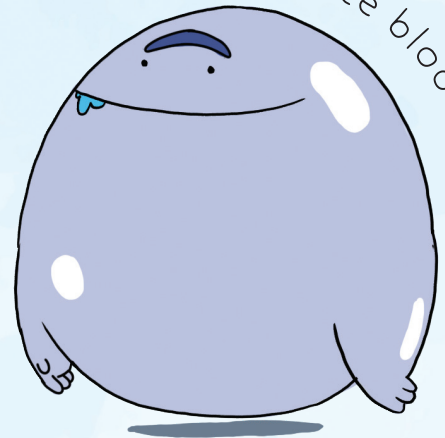
Virus
