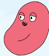
Cells
